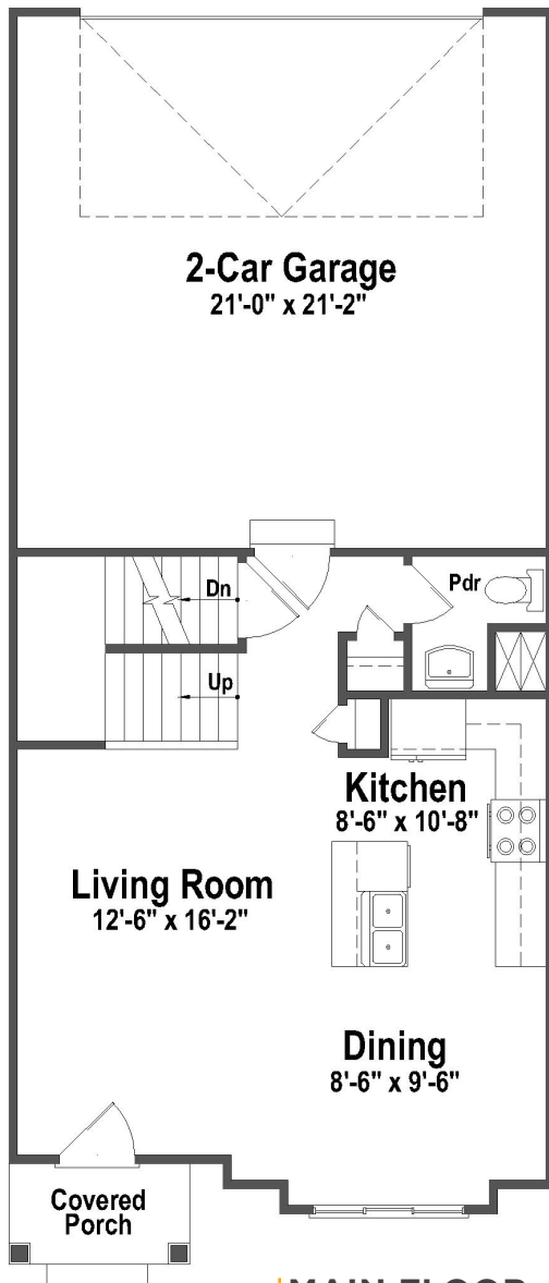
MAIN FLOOR Approx 560 Sq. Ft.
